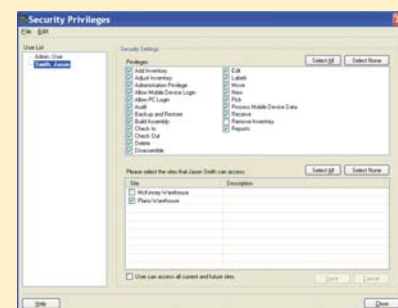
► Feature-based security
